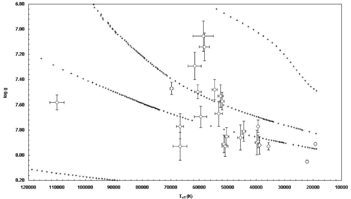
Figure 4. Values of T_{\text{eff}} and \log g measured from the Balmer lines for the sample of white dwarfs in this study. The crosses represent evolutionary tracks (from top to bottom) a He core white dwarf of 0.414 M_{\odot} and C/O core masses of 0.530, 0.605 and 0.836 M_{\odot} , calculated by Blöcker (1995) and Driebe et al. (1998).
