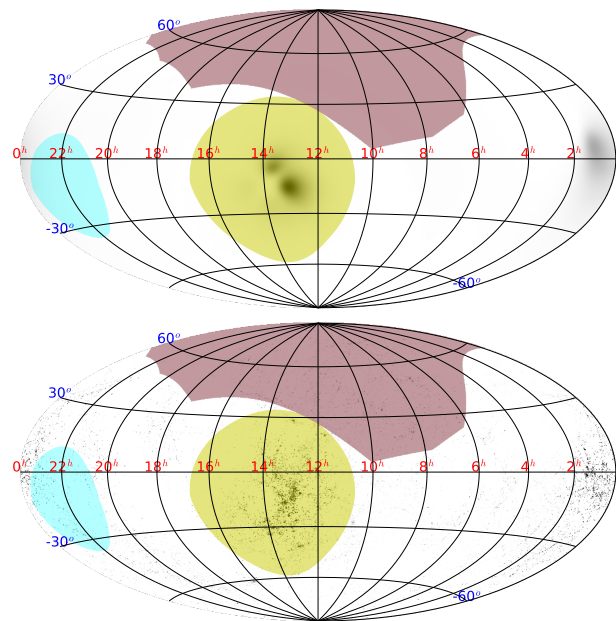
Figure 1. The ‘BAYESTAR’ GW localisation map for trigger G194575, produced by the LVC team on 2015 October 22 (top), combined with our luminosity-weighted GWGC map (bottom). Coordinates are equatorial, J2000. The yellow and cyan circles indicate the regions towards which XRT and UVOT cannot point due to proximity to the Sun and Moon respectively. The large maroon area is the BAT partially coded field of view at the time of the GW event. For this event, unfortunately the majority of the error region was unobservable due to its proximity to the Sun.
