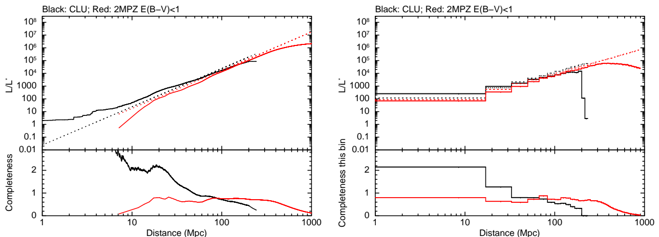
Figure 5. The completeness of the CLU (black) and 2MPZ V1.1 (red). In each plot the upper pane shows the theoretical total L/L^* predicted by a Schechter function (dotted line) as a function of distance, and the observed value from the catalogues (solid line); the lower pane shows the ratio of the theoretical to observed, which we interpret as the completeness of the catalogue. The CLU data and theoretical values relate to B -band magnitudes. The 2MPZ data use K -band magnitudes. For 2MPZ, only sources in regions with E(B - V) < 1 are included; the magnitudes have been corrected from isophotal to total values; see text for details. Left: Luminosity is integrated out to the distance on the x-axis, hence completeness refers to how complete the catalogue is out to distance D . Right: Luminosity is calculated in distance bins, hence completeness refers to how complete the catalogue is at distance D .
