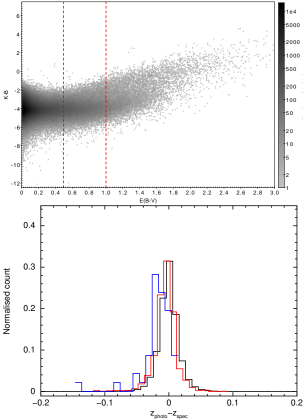
Figure 4. The effect of extinction on the colour and redshift accuracy of the 2MPZ V1.1 catalogue. Top: The extinction-corrected K-B colour as a function of extinction. For values of E(B-V) \geq 0.5 a clear trend starts to emerge, indicating a selection effect due to reddening. The contours indicate the density of the points, and the red lines mark E(B-V) = 0.5 and 1. Bottom: Histograms of z_{\text{photo}} - z_{\text{spec}} for objects with spectroscopic redshift measurements, for E(B-V) < 0.5 (black), 0.5 \leq E(B-V) < 1 (red) and E(B-V) \geq 1 (blue). The red histogram shows a small systematic shift, such that the mean photometric redshift is 0.004 too low compared to spectroscopic values; the widths are comparable. At high extinction, the photometric redshift calibration becomes very poor.
