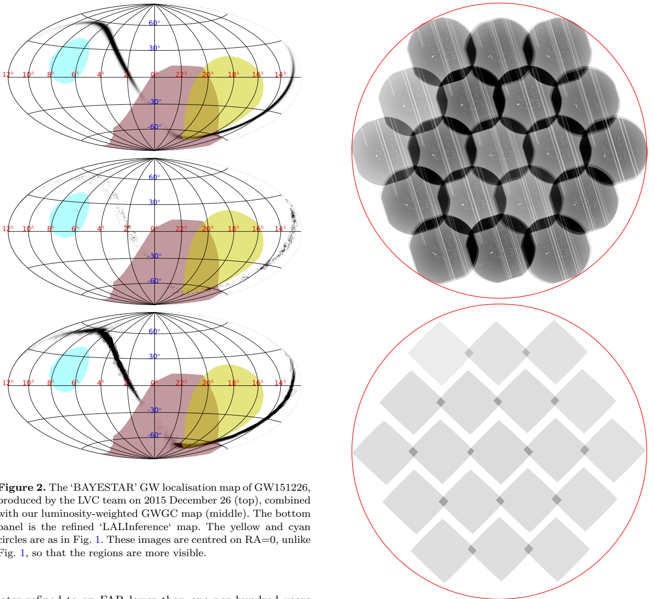
Figure 3. An example XRT (top) and UVOT (bottom) exposure map from a 19-point tile used in the follow-up observations of GW151226. The circle is shown for scale and has radius 0.88°.
